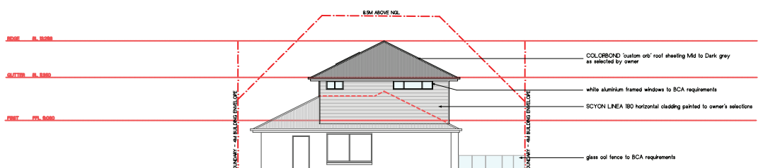
SOUTH ELEVATION
