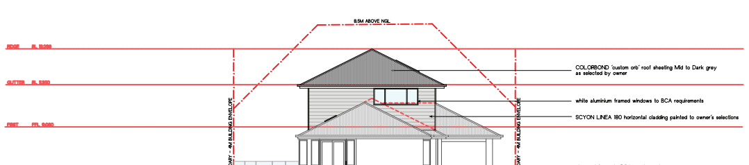
NORTH ELEVATION
