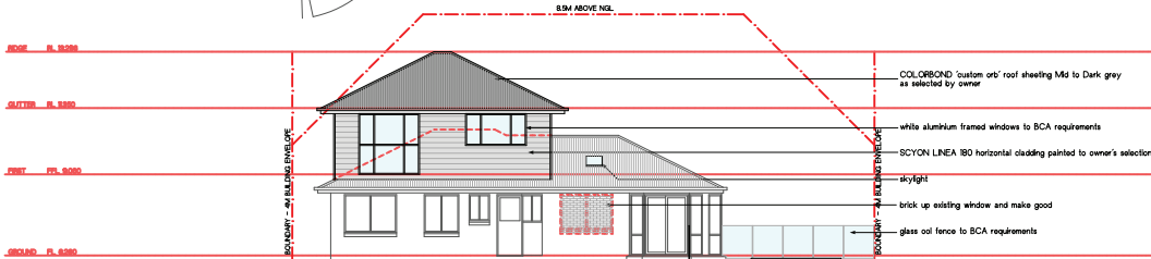
EAST ELEVATION
