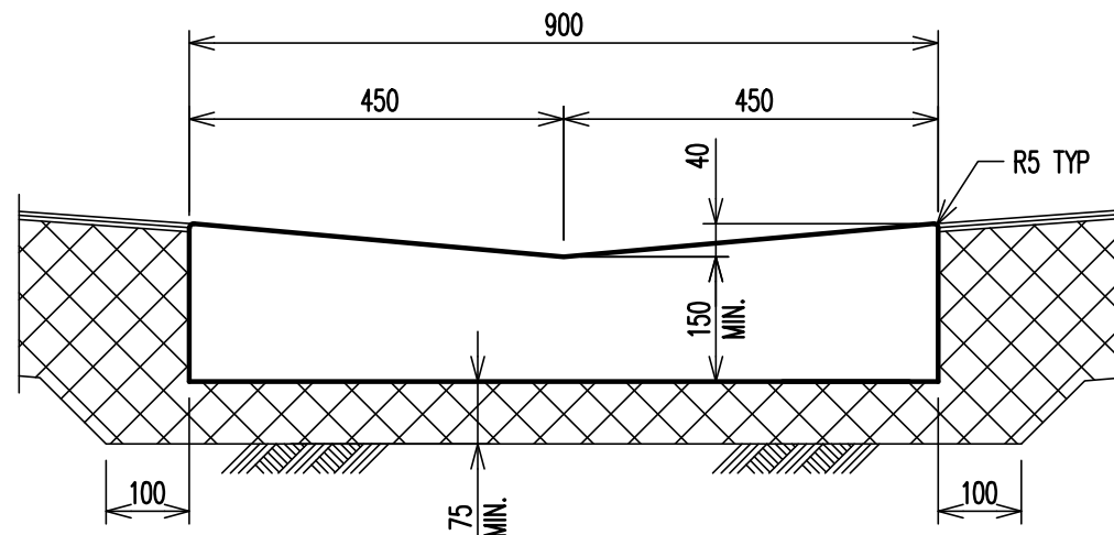
DISH DRAIN (DD) SCALE 1:10
