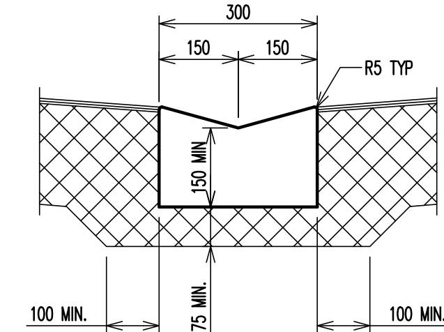
DISH DRAIN TYPE A (DDA) SCALE 1:10
