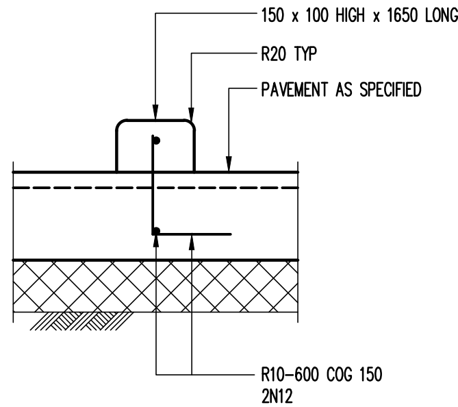
WHEEL STOP IN CONCRETE PAVEMENT SCALE 1:10
