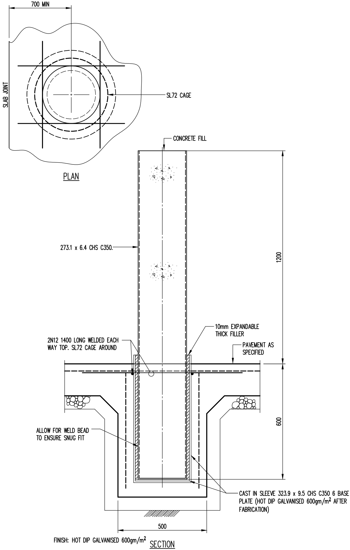
BOLLARD TO CONCRETE PAVEMENT SCALE 1:10
