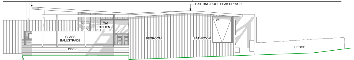
South Elevation - Proposed
