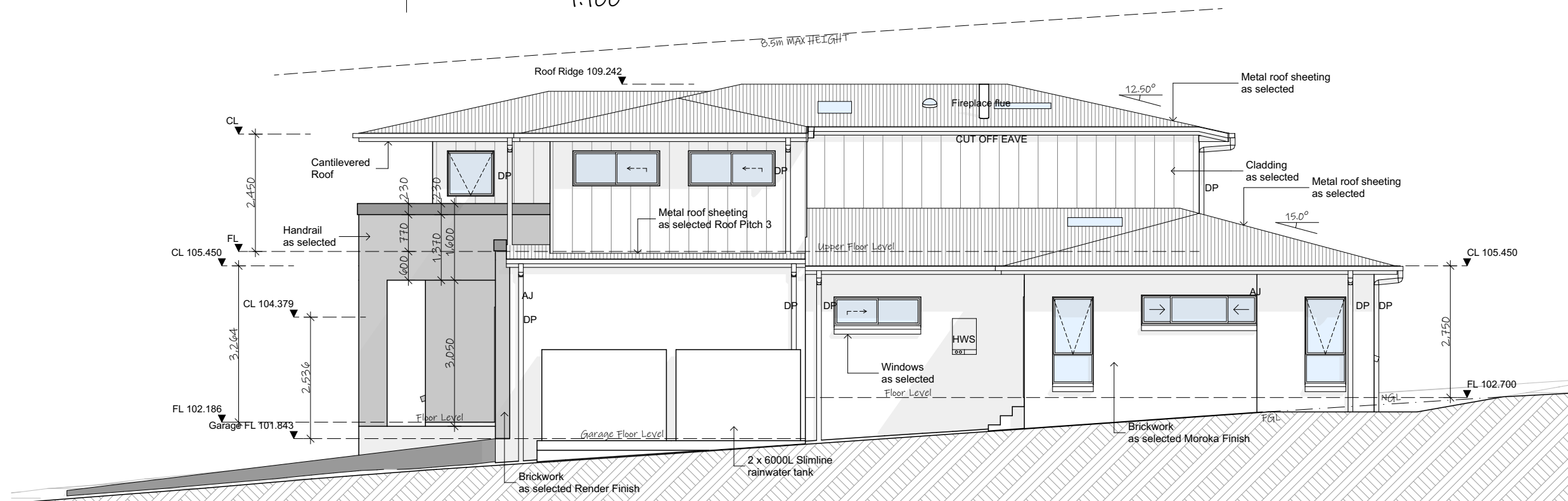
West/Side Elevation 1:100
