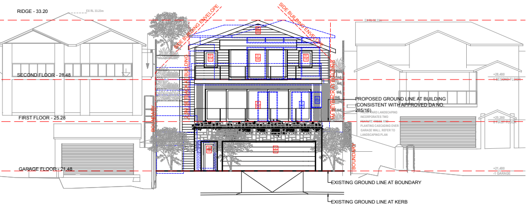
NORTH ELEVATION
