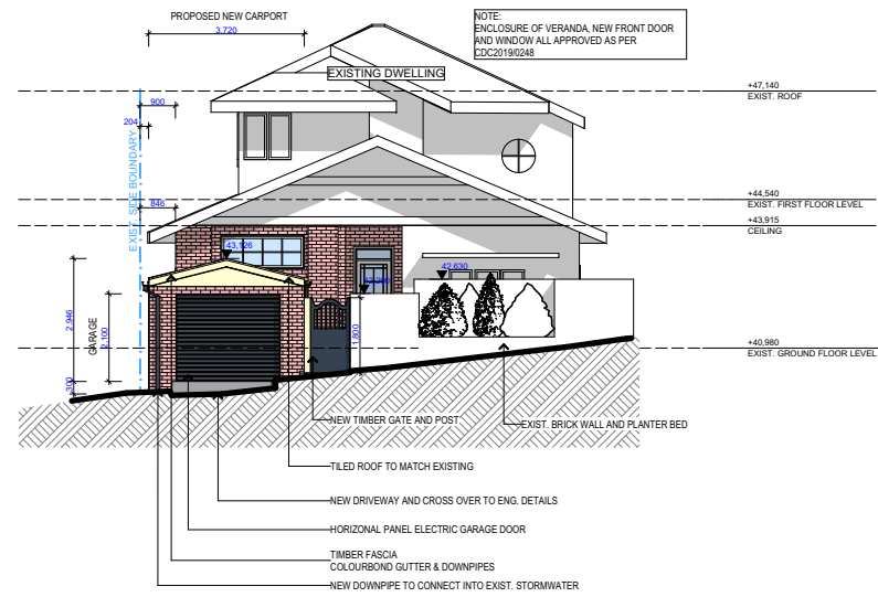
NORTH ELEVATION 1:200
