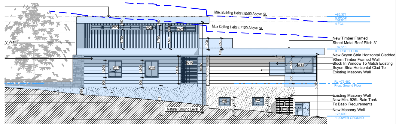
East 1:200
