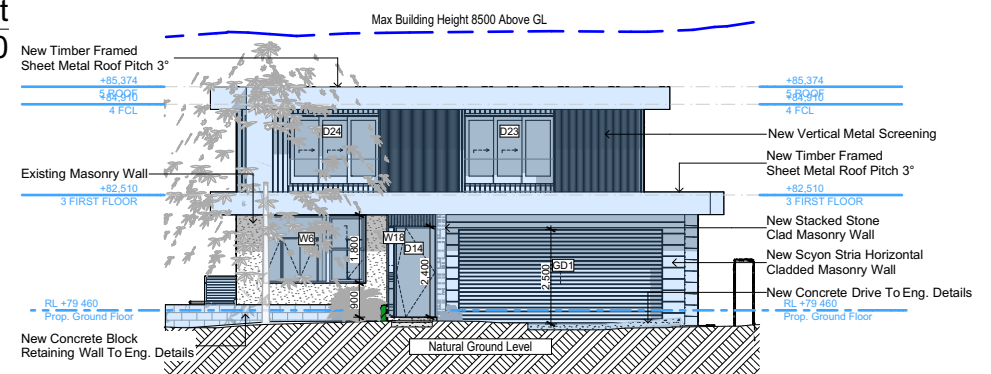
South 1:200
