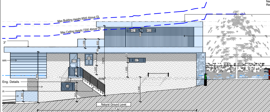
West 1:200
