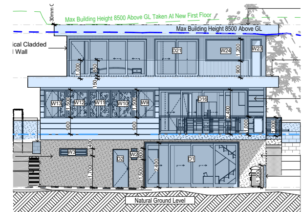
North 1:200
