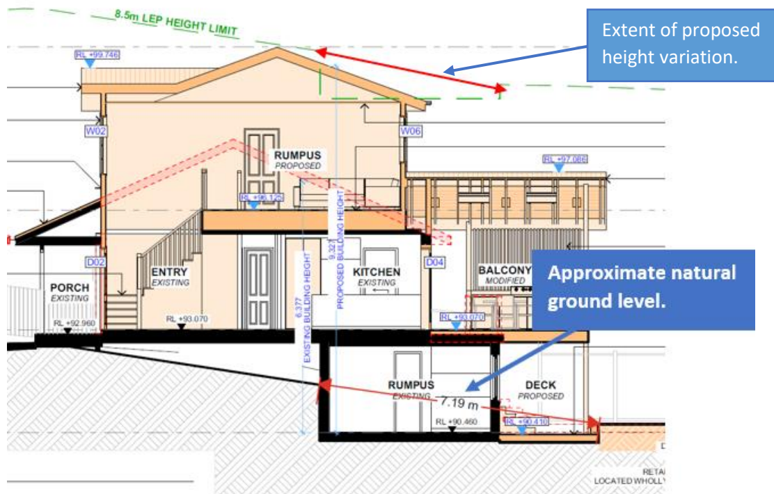
Figure 1: Extract from architectural plans shows the extent of the proposed variation.
