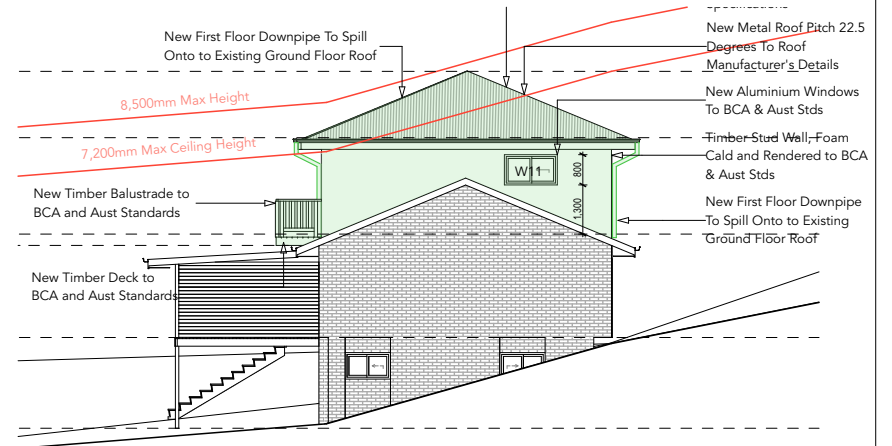
South Elevation
