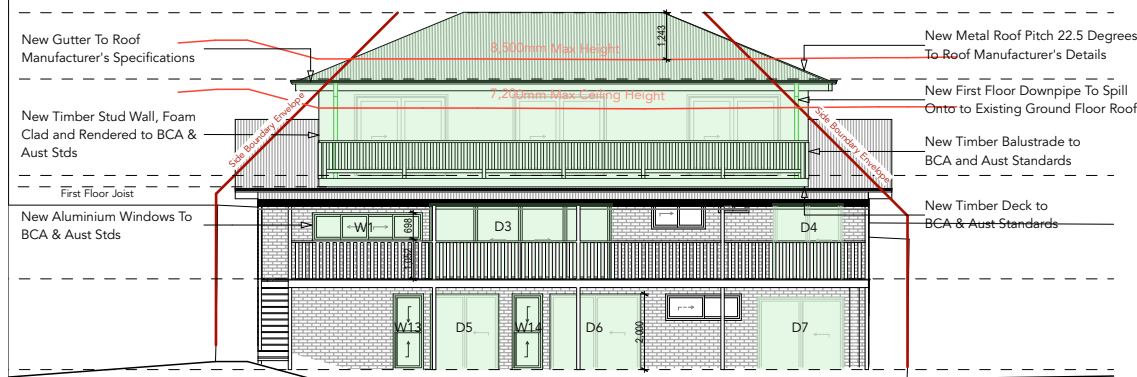
West Elevation
