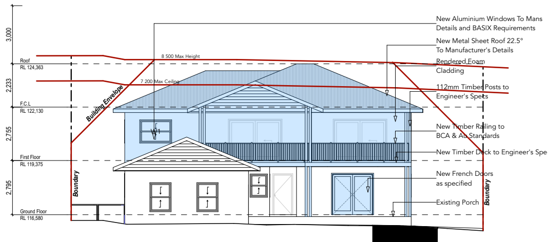
North Elevation
