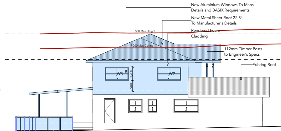
East Elevation
