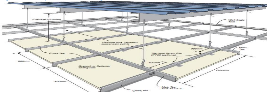
Figure 4.2 Example of Internal Ceiling Construction with Plasterboard
