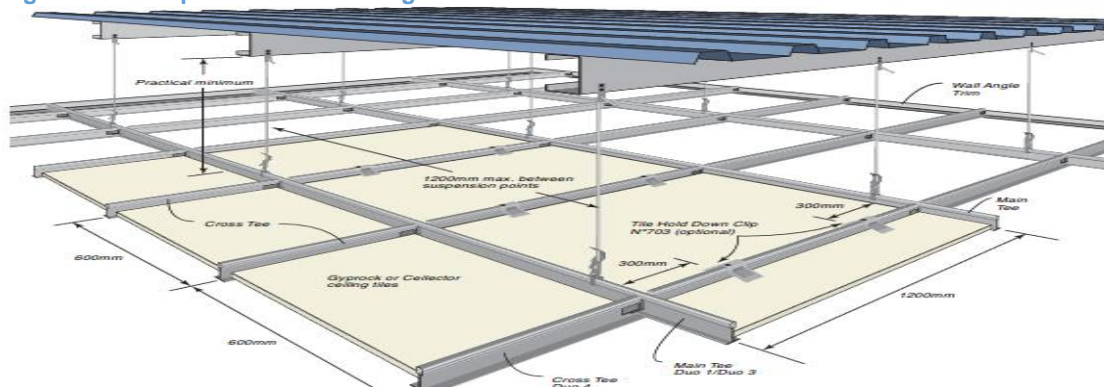
Figure 4.1 Example of Internal Ceiling Construction with Plasterboard
