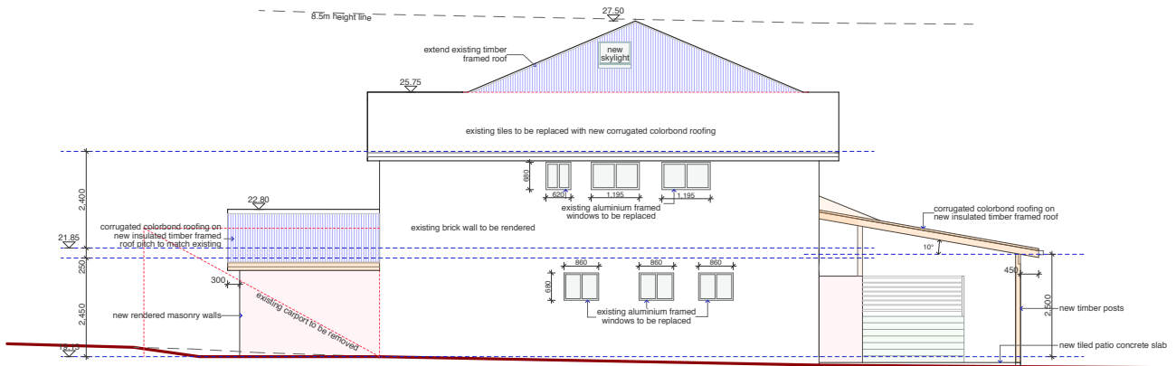
WEST ELEVATION
