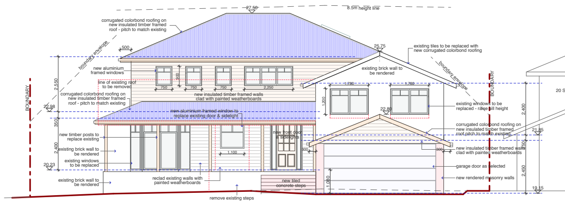
WEST ELEVATION
