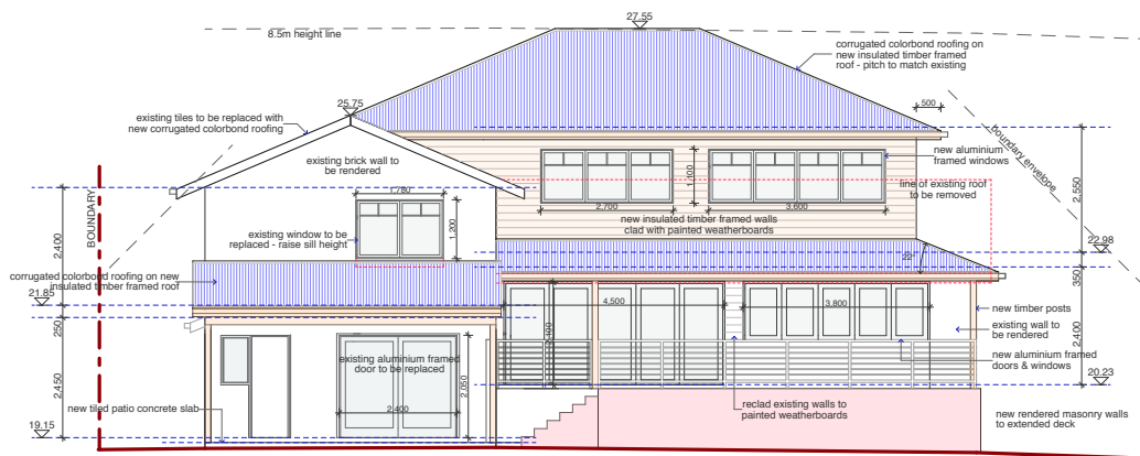
EAST ELEVATION
