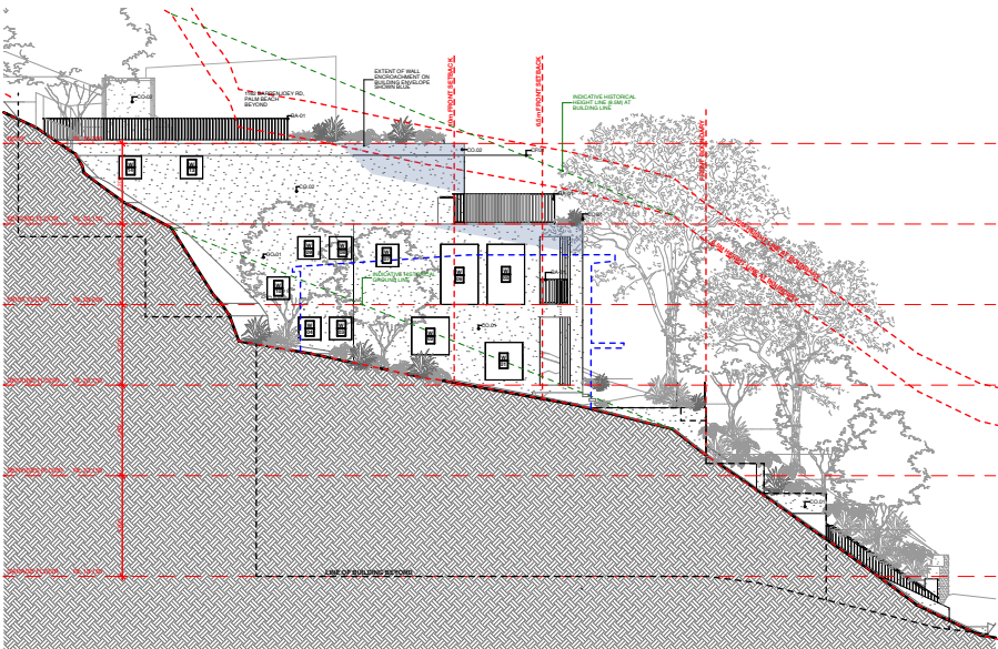
EAST ELEVATION
