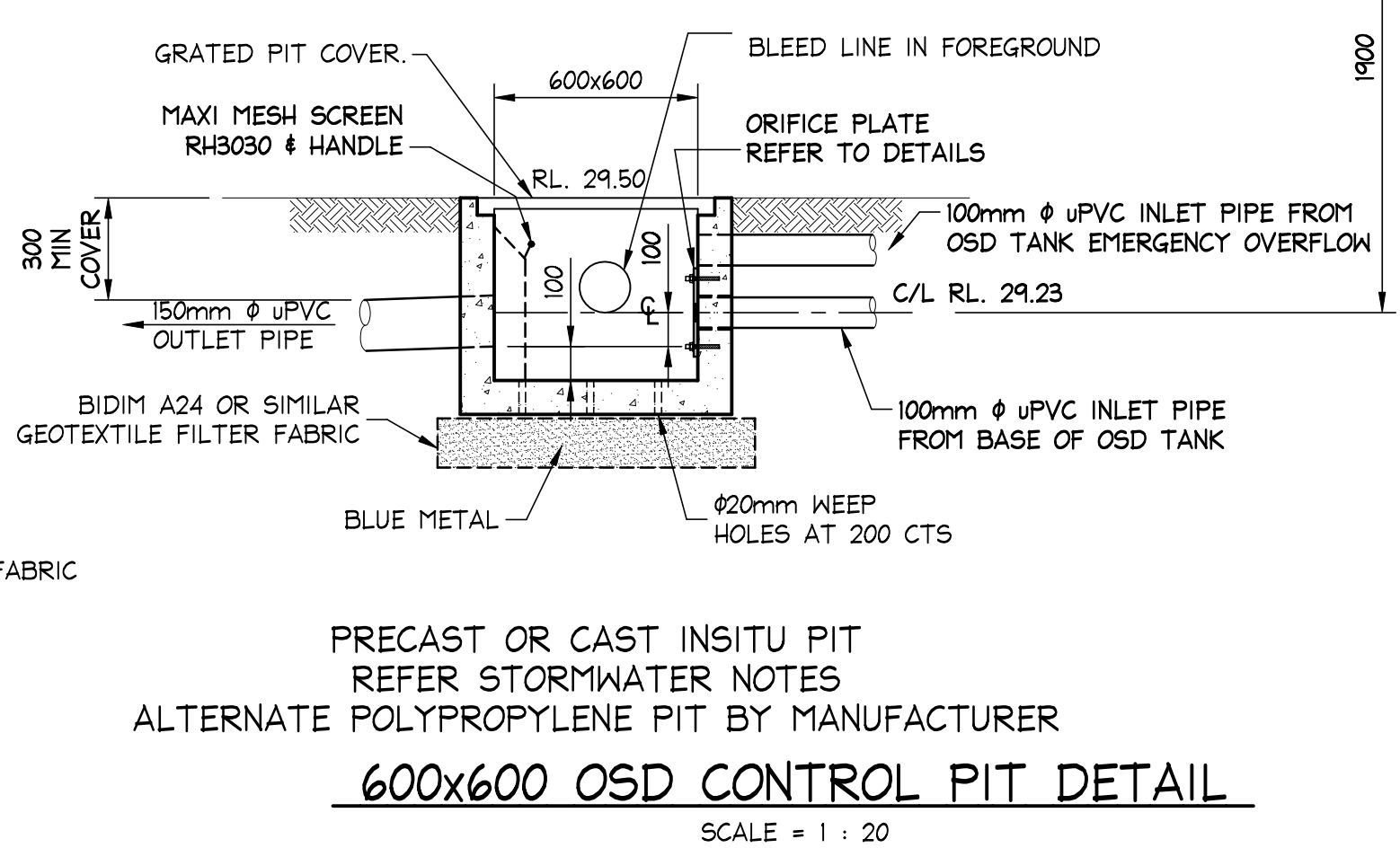
PRECAST OR CAST INSITU PIT REFER STORMWATER NOTES 600x600 FLUSH OUT PIT DETAIL SCALE = 1 : 20
