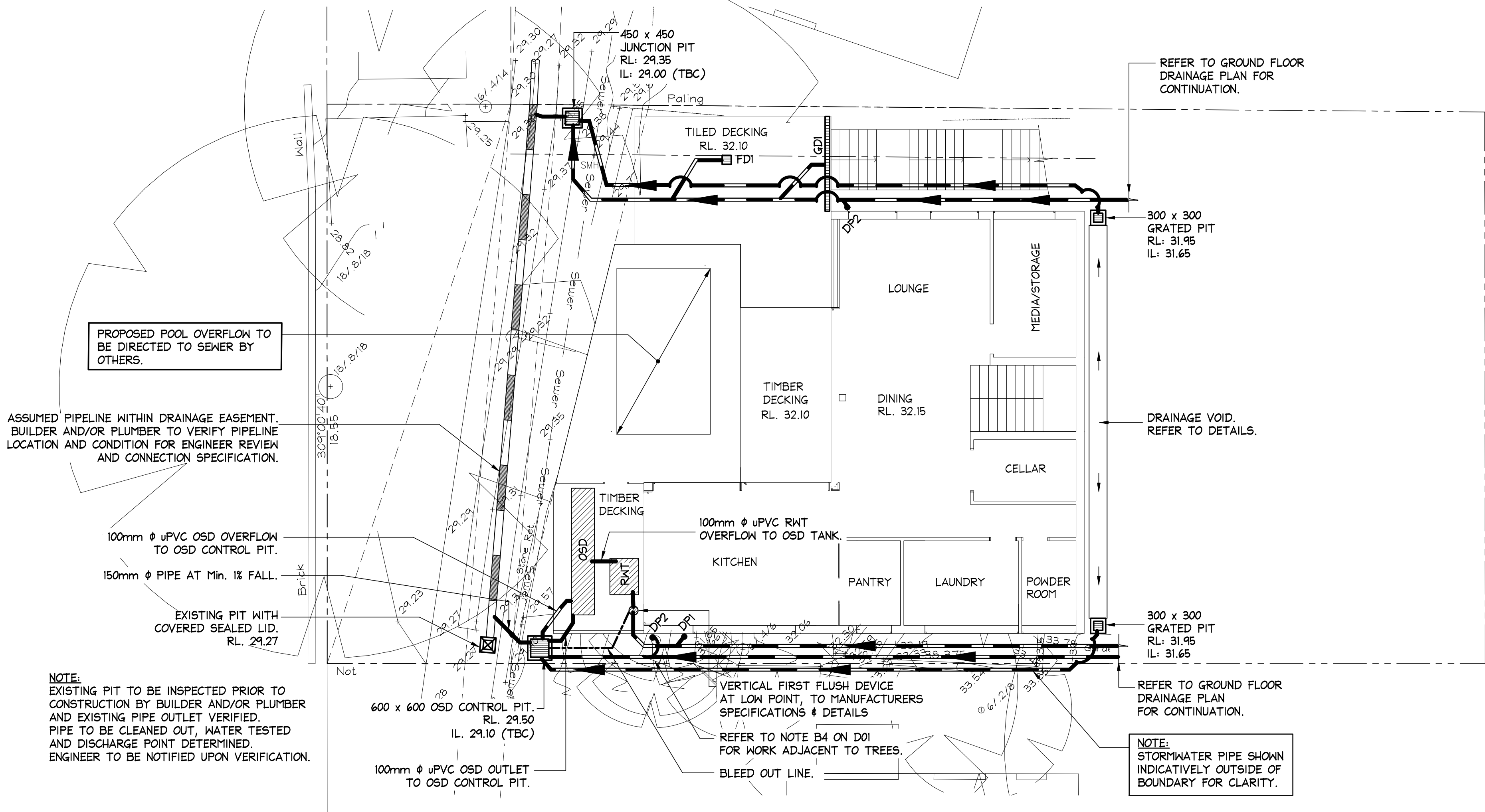
LOWER GROUND FLOOR AND SITE DRAINAGE MANAGEMENT PLAN SCALE = 1:100
