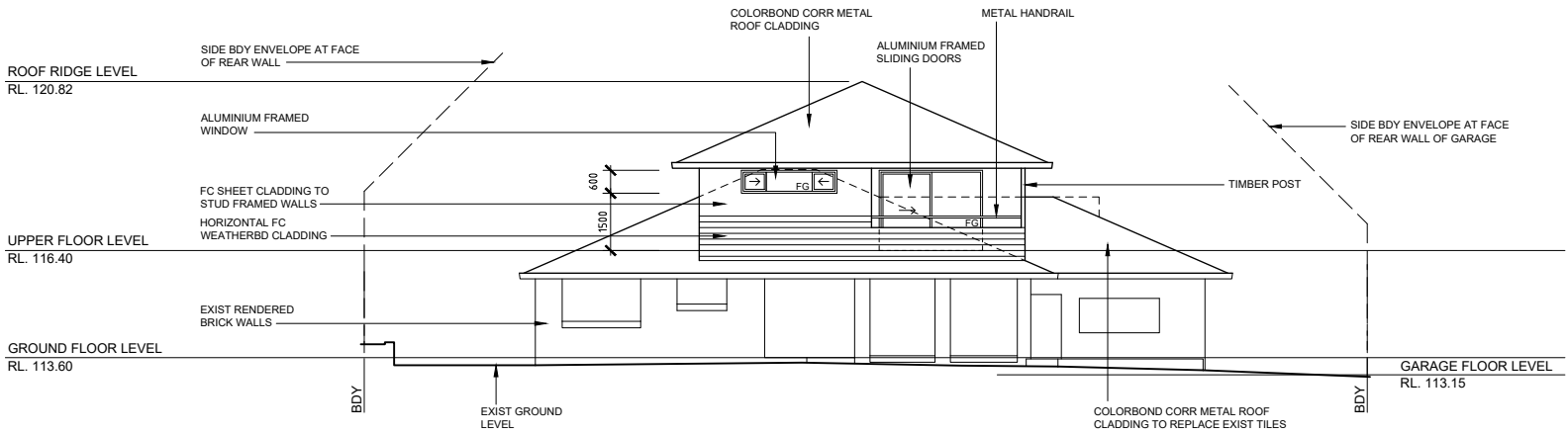
EAST ELEVATION
