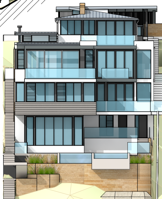
3 WEST ELEVATION Scale 1:200
