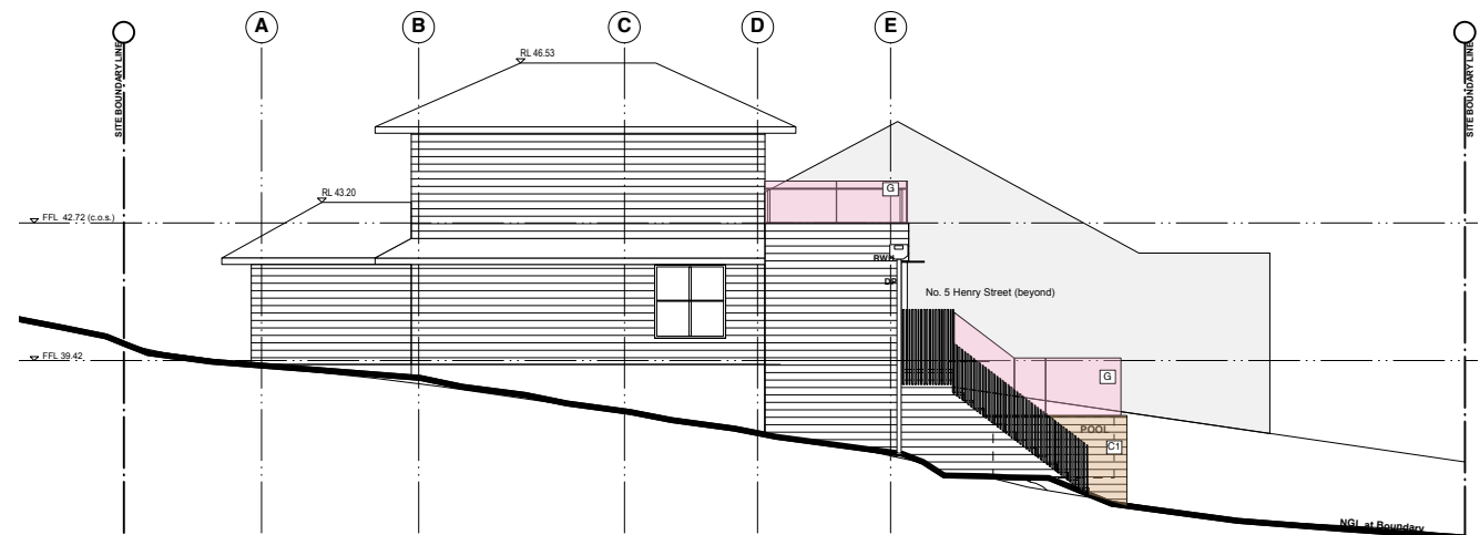
04 Side Elevation I EAST
