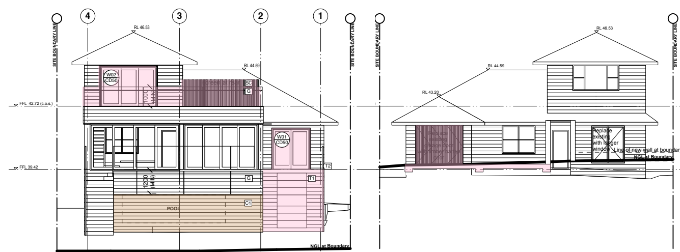
02 Rear Elevation I NORTH 03 Front Elevation I SOUTH
