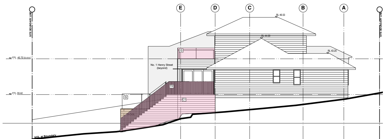
05 Side Elevation I WEST
