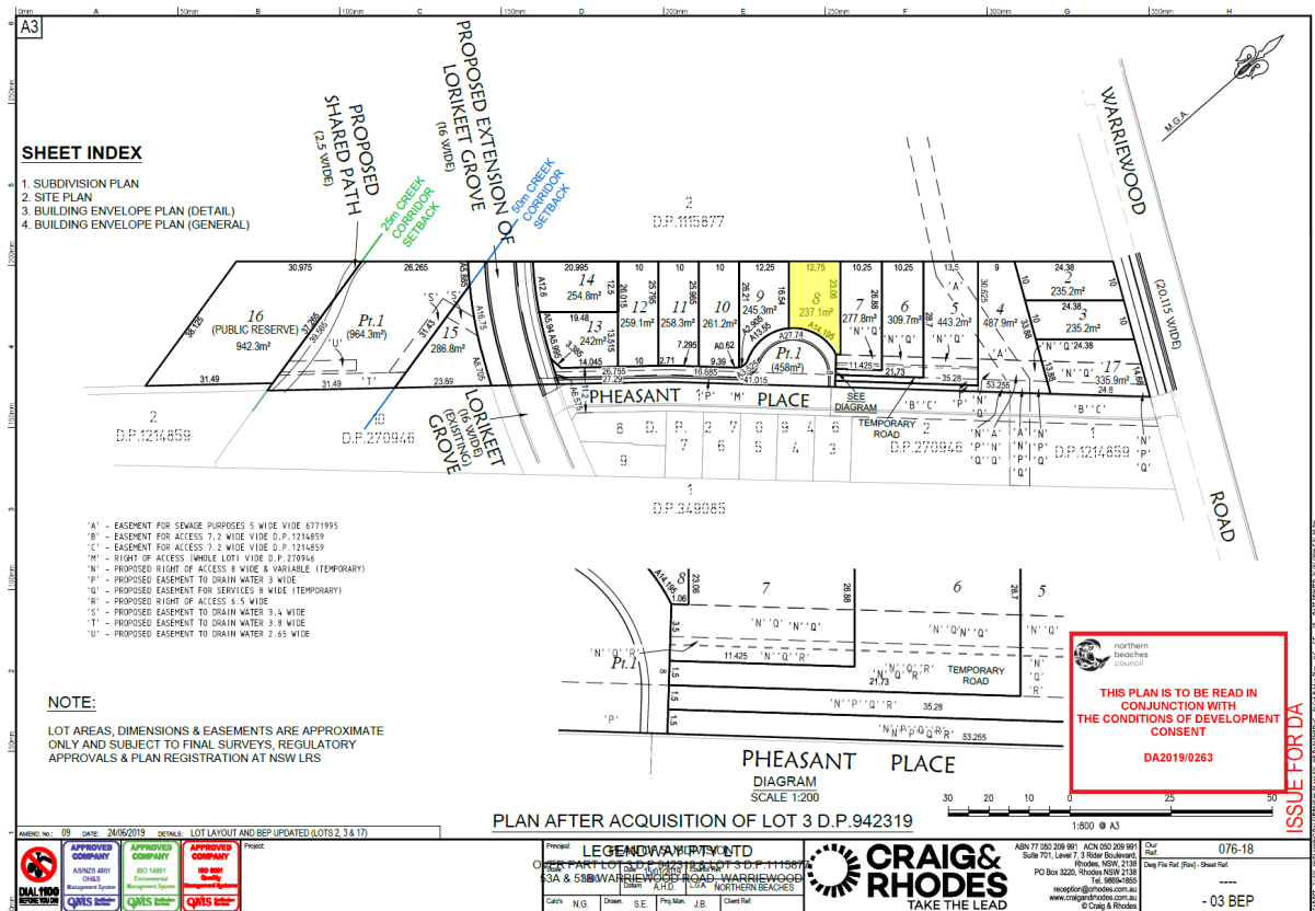
Figure 2 – Approved Subdivision Plan DA2019/0263 with Lot 8 highlighted in yellow Source: Northern Beaches Council
