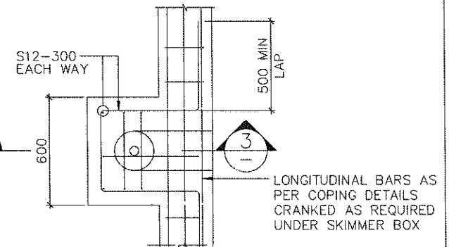
PLAN OF SKIMMER 1:20
