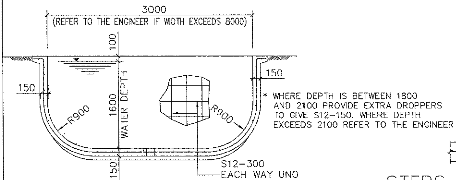
DEEP END SECTION 1:50
