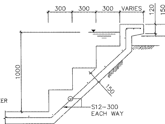
STEPS CAST AGAINST GROUND 1:20
