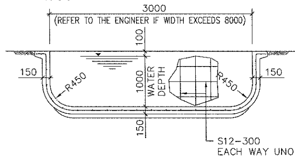
SHALLOW END SECTION 1:50
