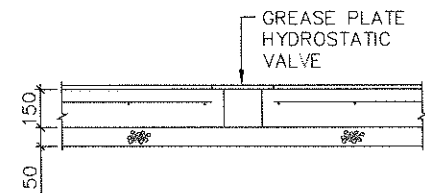
HYDROSTATIC VALVE DETAIL 1:20
