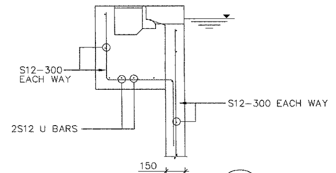
SECTION 1:20
