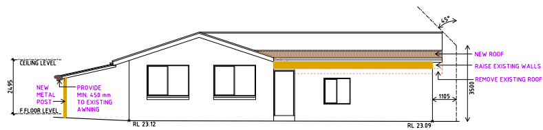
SOUTH EAST ELEVATION SCALE 1:100
