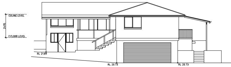
NORTH WEST ELEVATION SCALE 1:100
