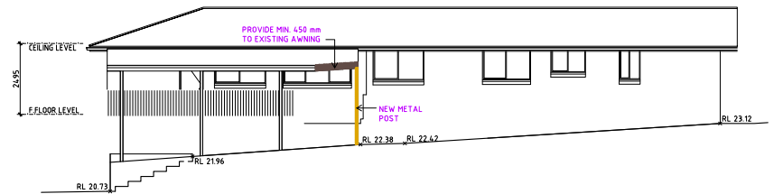
SOUTH WEST ELEVATION SCALE 1:100
