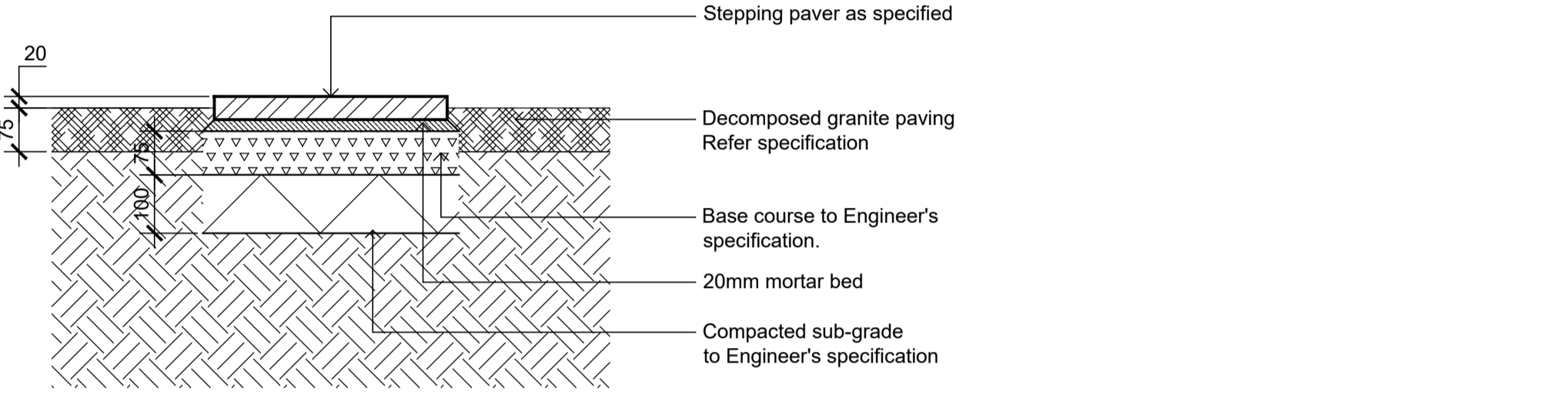
5 STEPPING PAVER IN DECOMPOSED GRANITE ON GRADE SCALE 1:10
