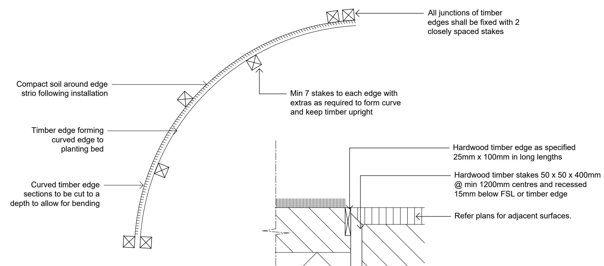
4 TIMBER EDGE - PLAN & SECTION SCALE 1:10
