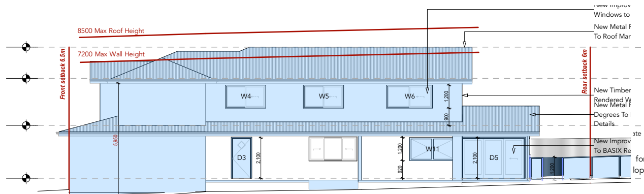
South Elevation
