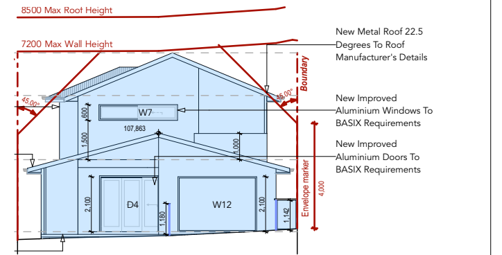
East Elevation
