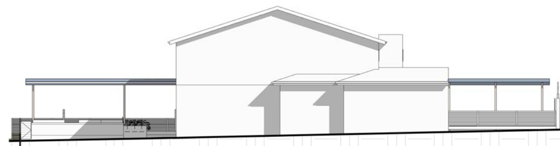
4 SOUTH EAST ELEVATION 1 : 250
