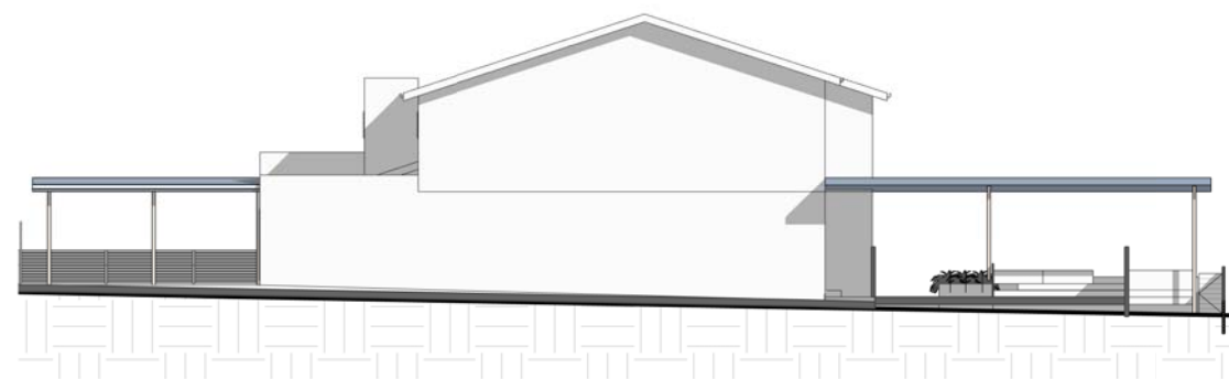
3 NORTH WEST ELEVATION 1 : 250
