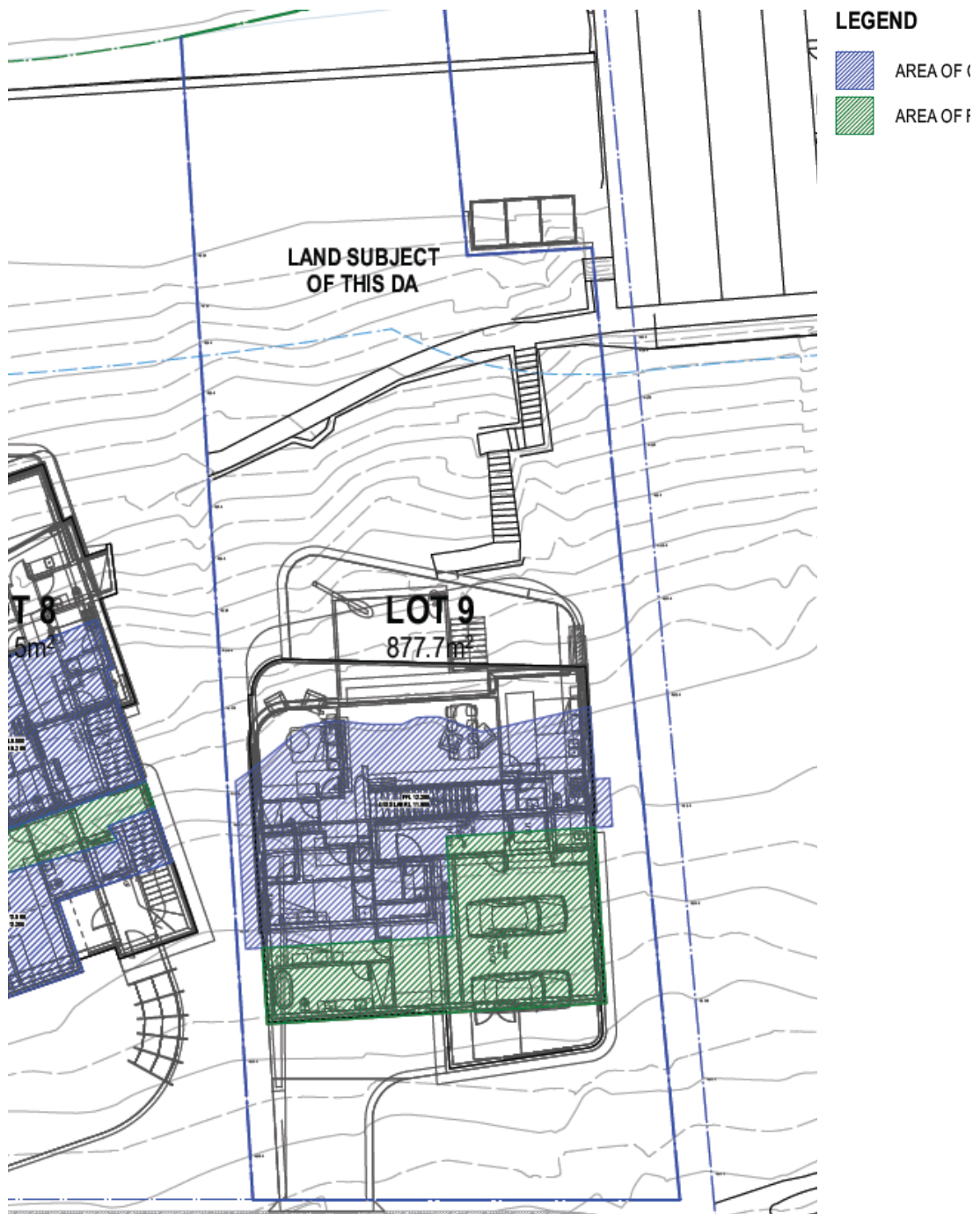
Figure 24 – areas of proposed cut and fill
