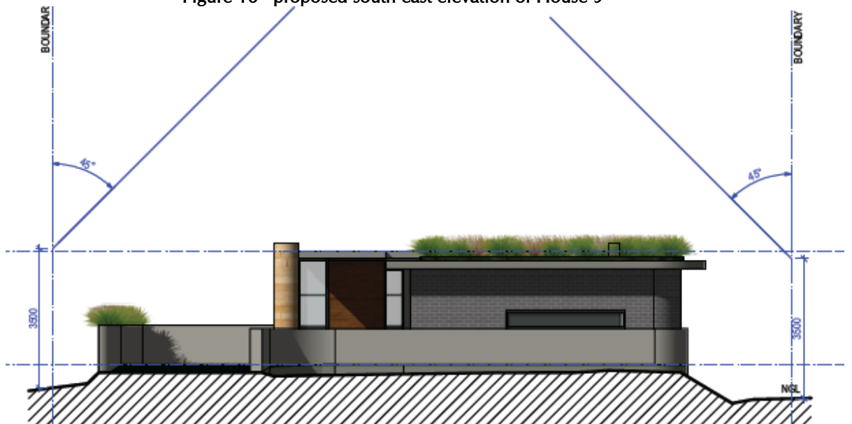
Figure 17– proposed south-west elevation of House 9
