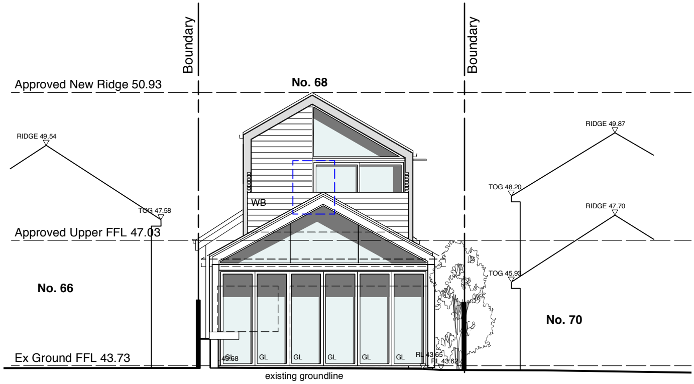
East Elevation
