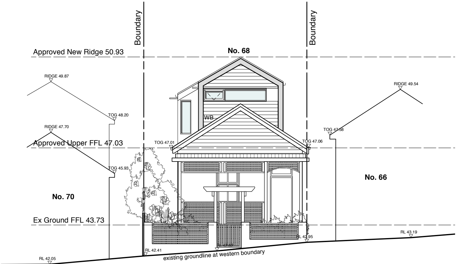
West/Street Elevation
