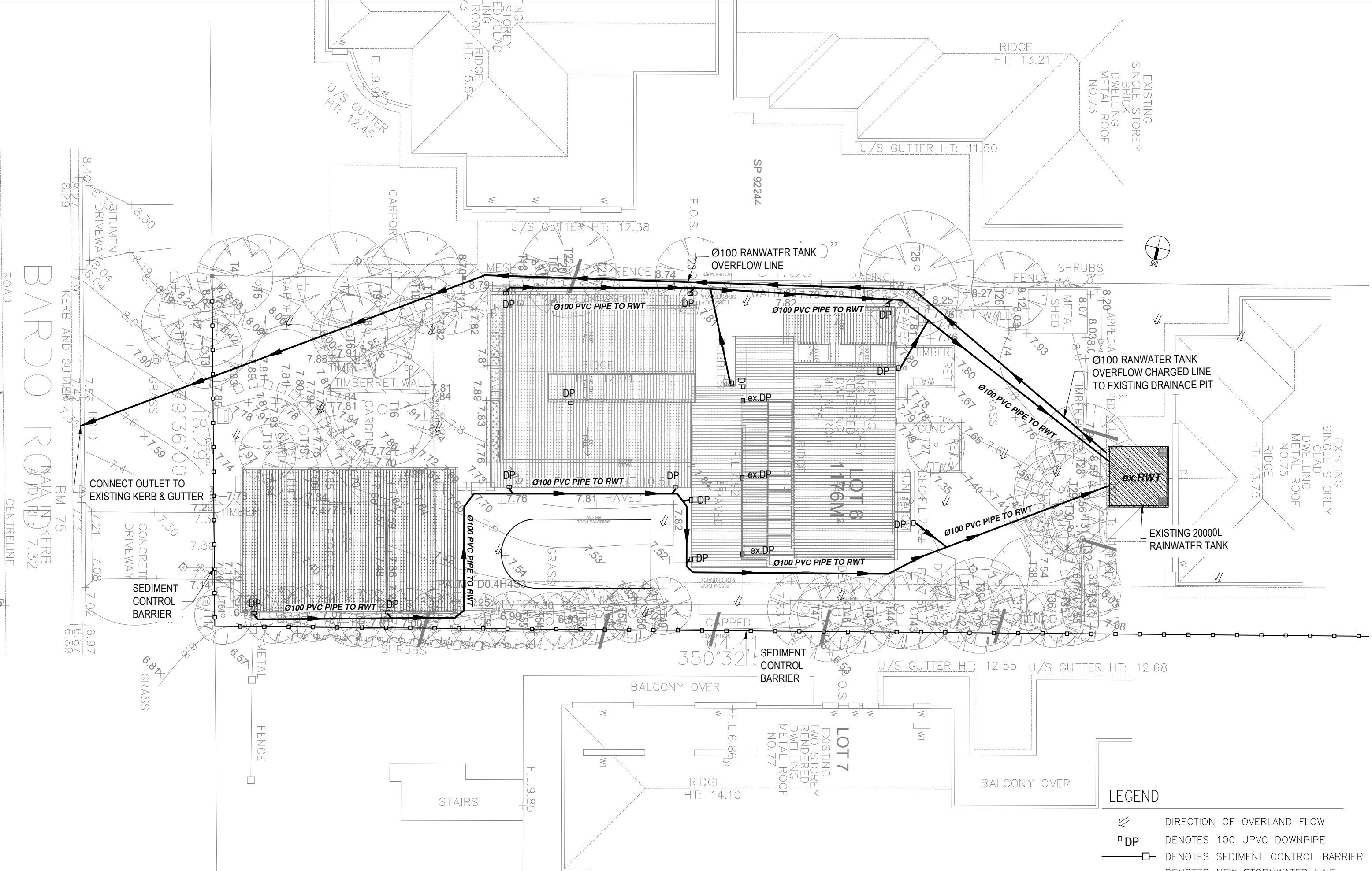
DRAINAGE PLAN SCALE 1:175
