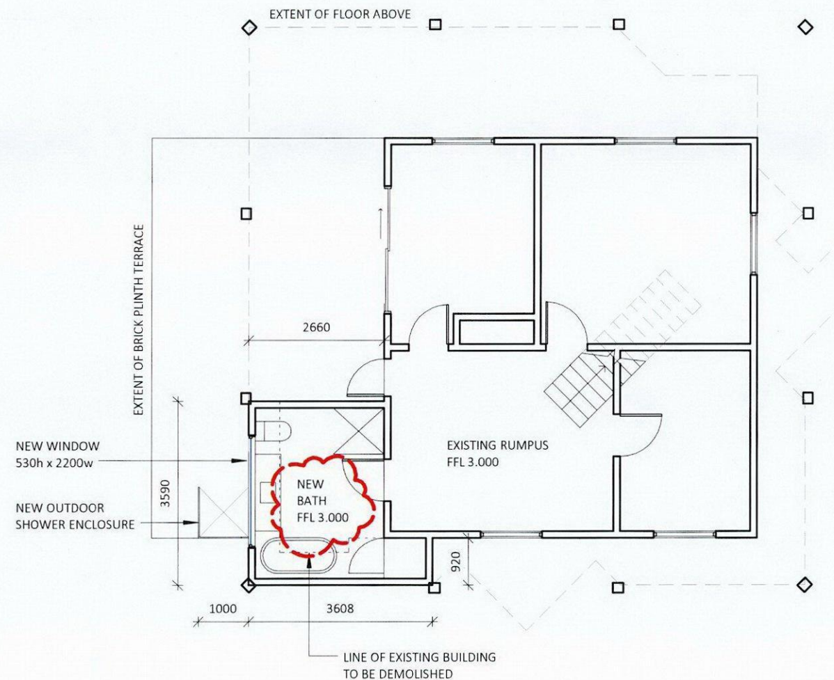
2 LEVEL 1 PROPOSED 1 : 100
