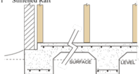
Fig. 1 Stiffened Raft
