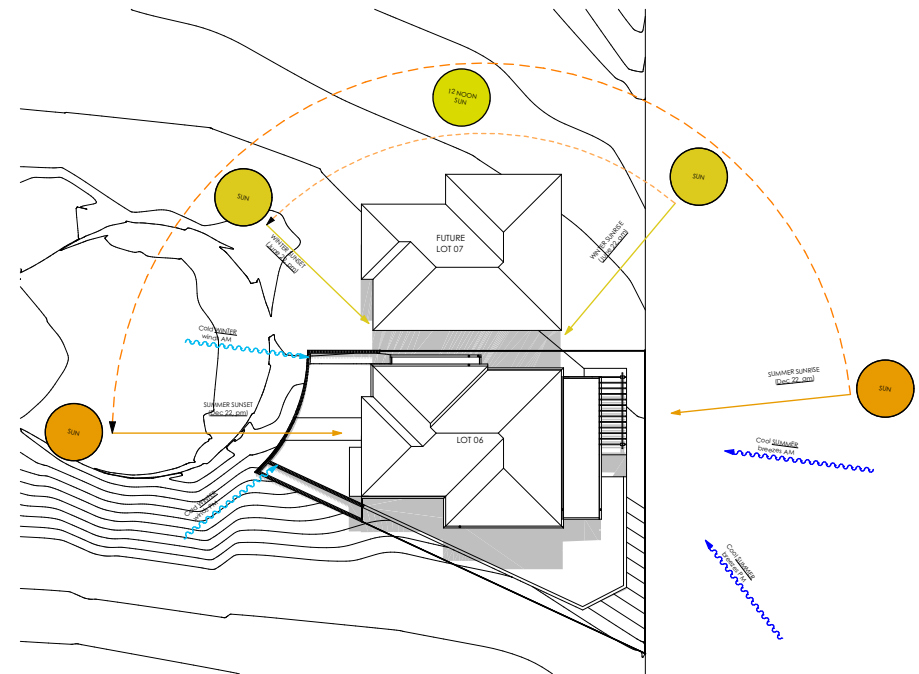
5 SITE ANALYSIS PLAN 1:500
