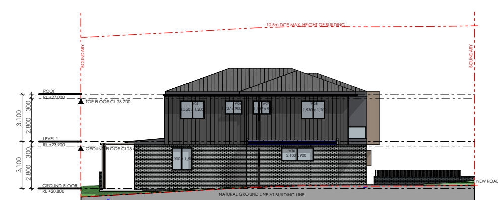
2 NORTH ELEVATION 1:250
