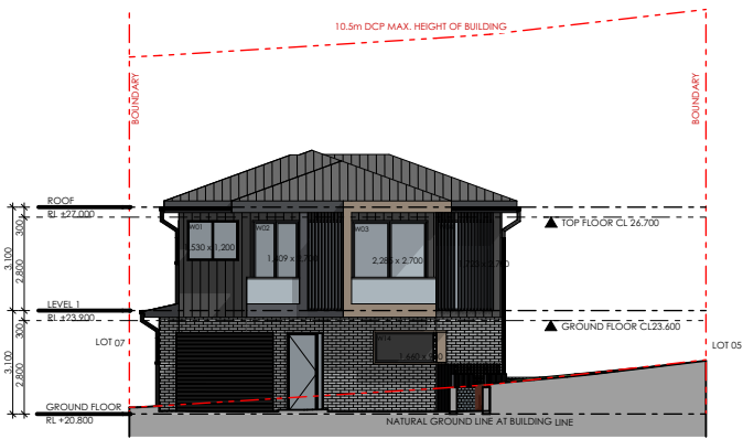
1 WEST ELEVATION 1:250
