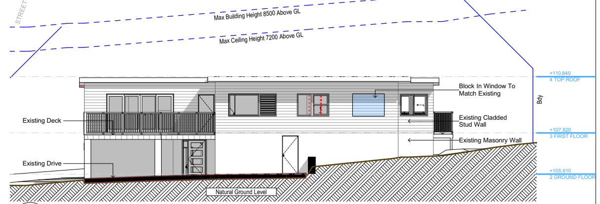
E-02 East 1:200
