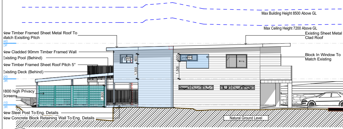
E-03 South 1:200
