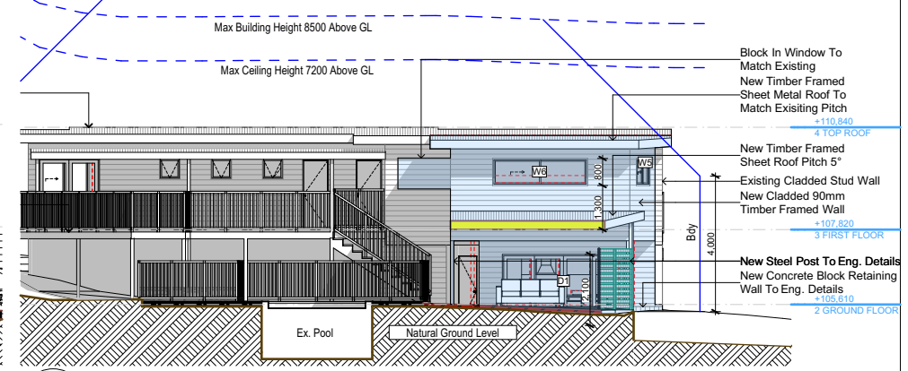
E-04 West 1:200
