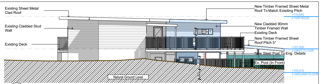
E-01 North 1:200
