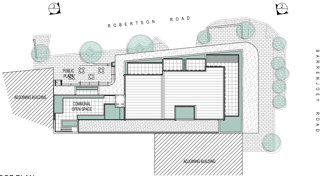
1 SITE & ROOF PLAN
