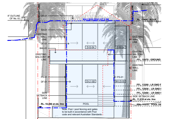
5 West Elevation Proposed 1:200
