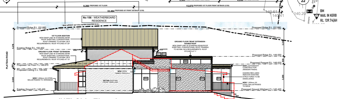
(NE) Side Elevation
