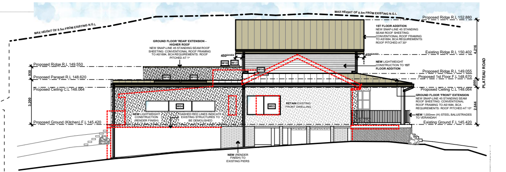
(SW) Side Elevation
