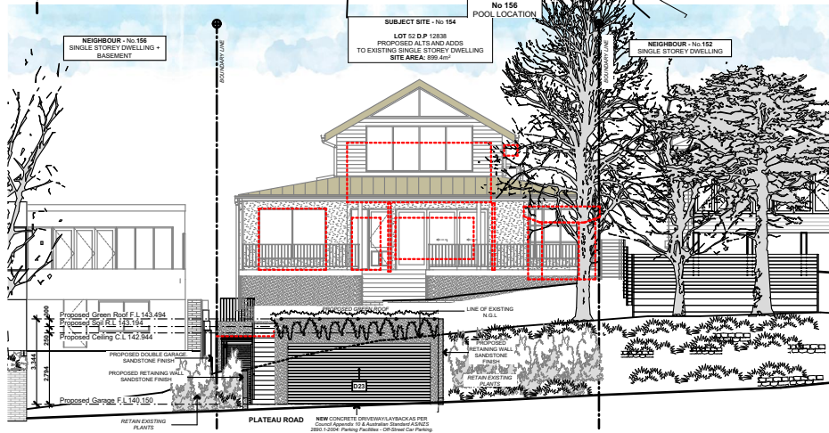
(SE) Front Elevation
