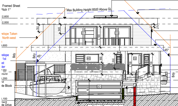
North 1:200
