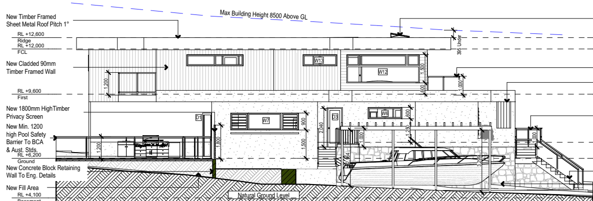
East 1:200
