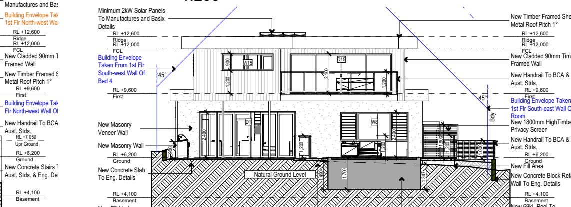
South 1:200
