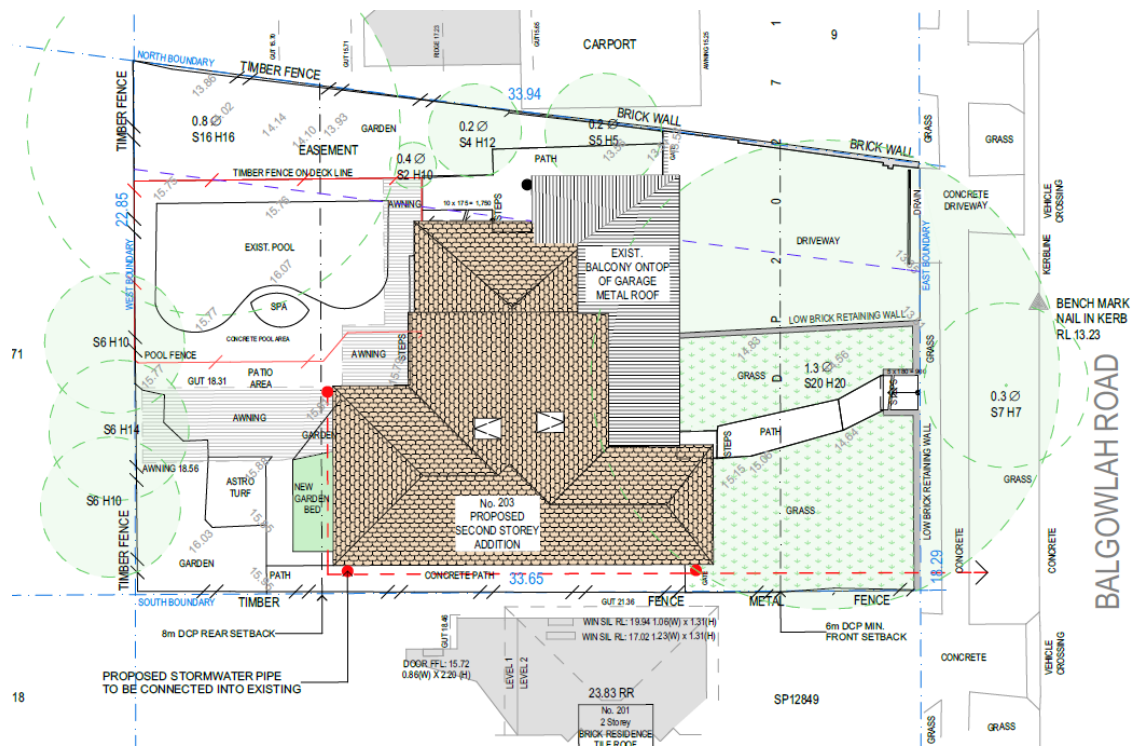
Figure 2: Site Plan.
