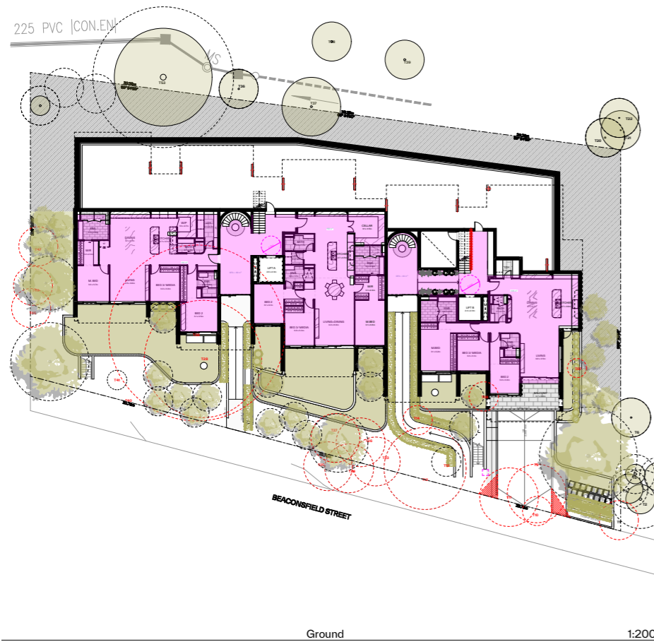
Ground 1:200
