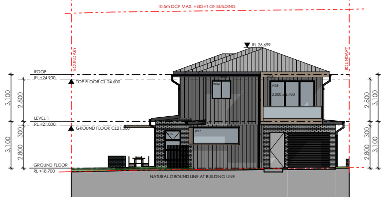
1 WEST ELEVATION 1:250
