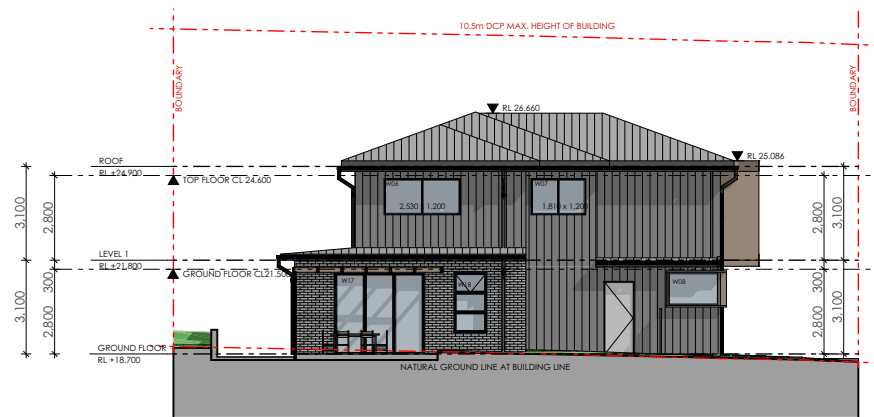
2 EAST ELEVATION 1:250
