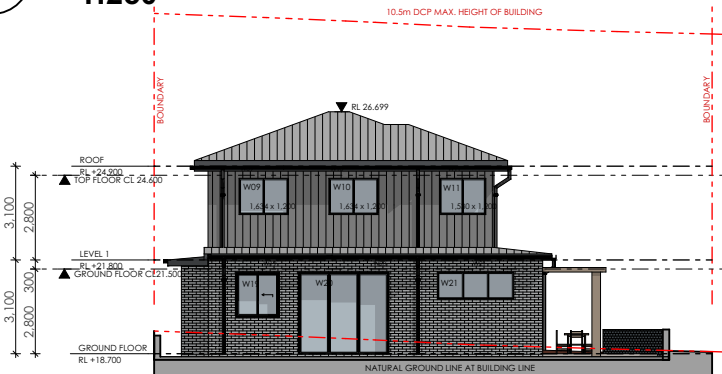
4 SOUTH ELEVATION 1:250
