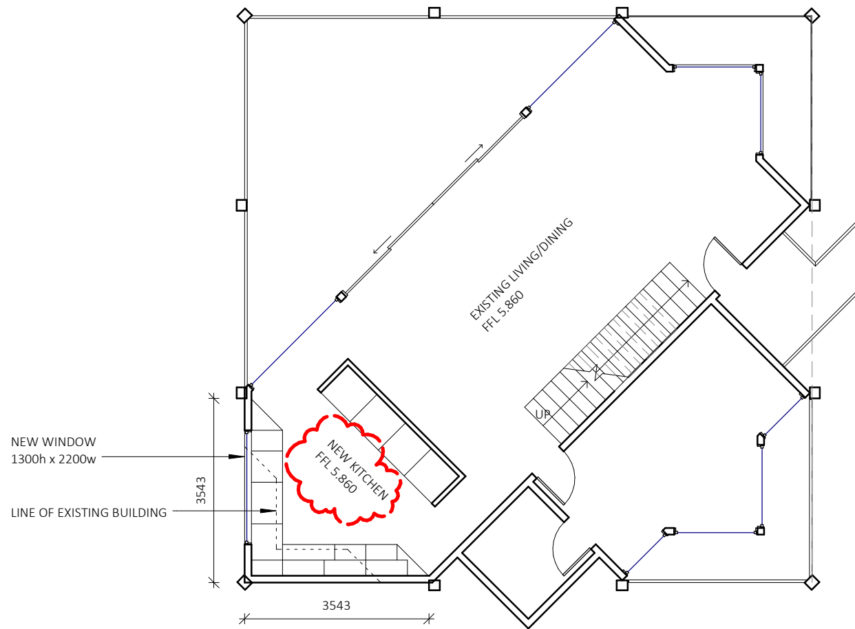
2 LEVEL 2 PROPOSED 1 : 100
