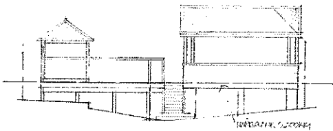
WEST ELEVATION
