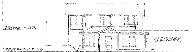
EAST ELEVATION
