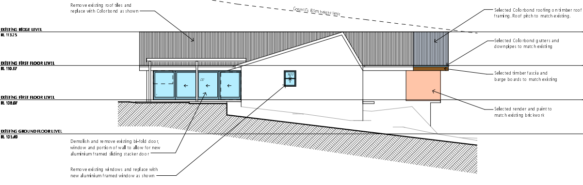
2 NORTH ELEVATION 1:100
