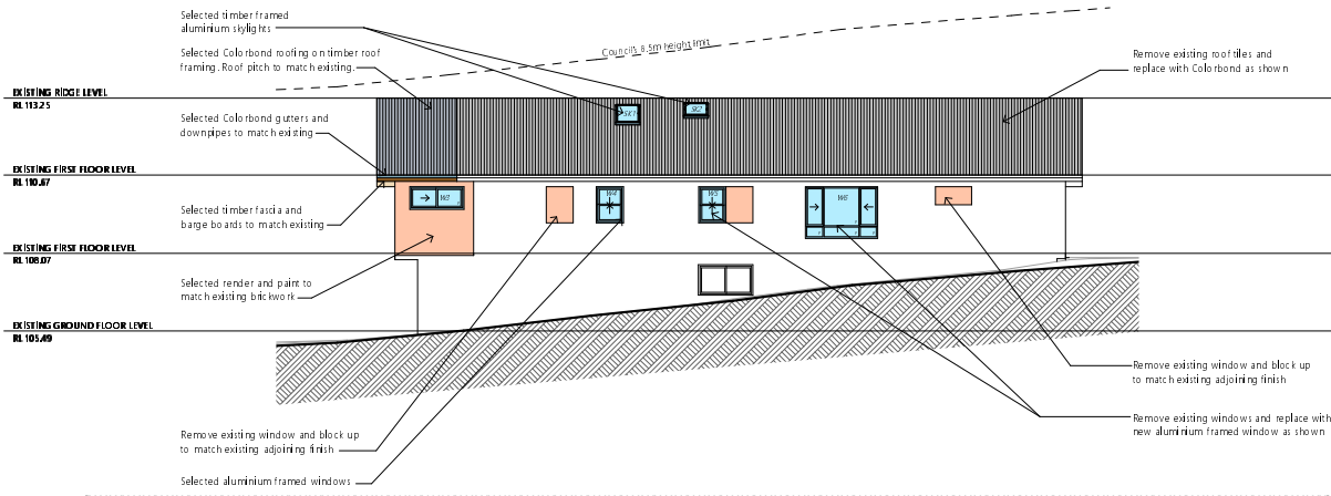
1 SOUTH ELEVATION 1:100
