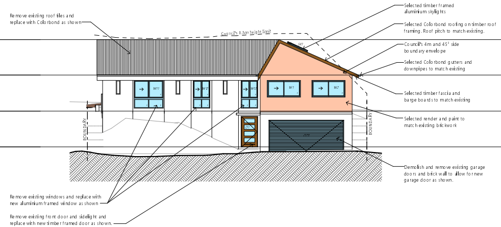
3 WEST ELEVATION 1:100
