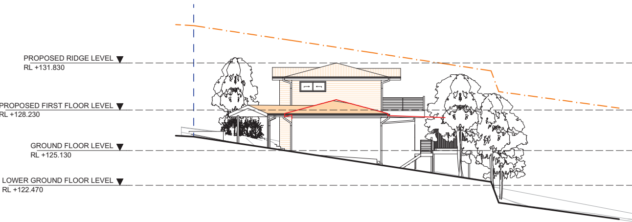
2 SOUTH ELEVATION 1:200
