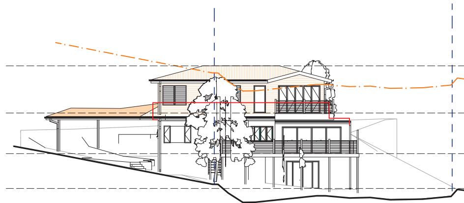
3 EAST ELEVATION 1:200
