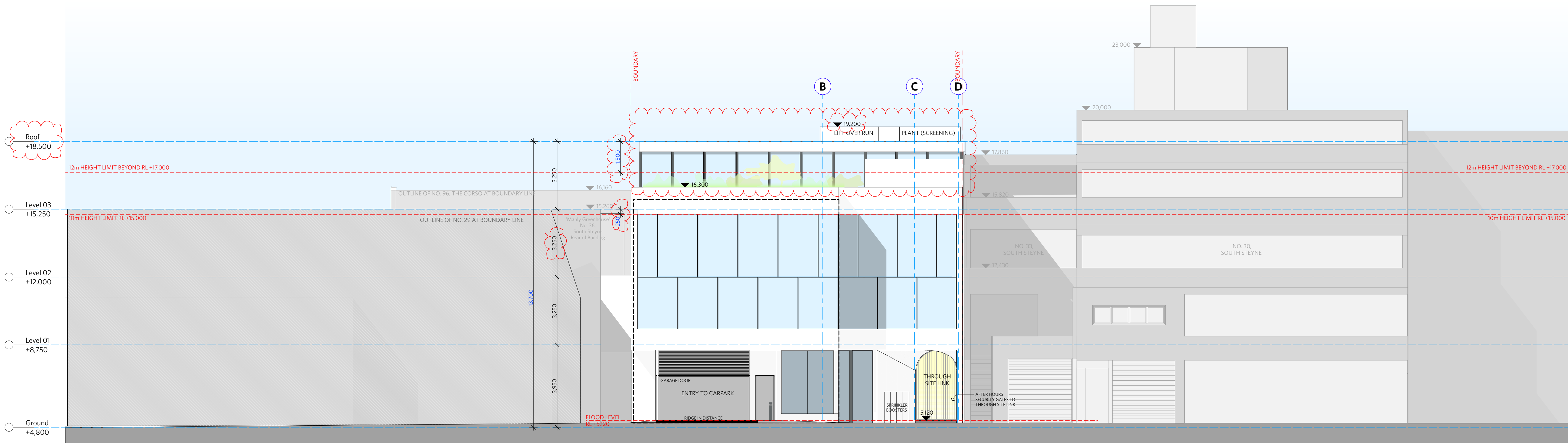
West Elevation
