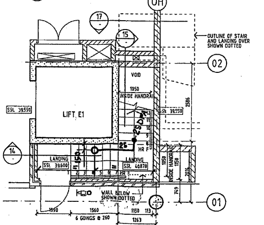
09 LEVEL 01 PLAN STAIR E-02
