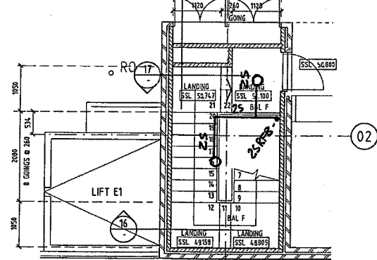
12 LEVEL 04 (ROOF) PLAN STAIR E-02
