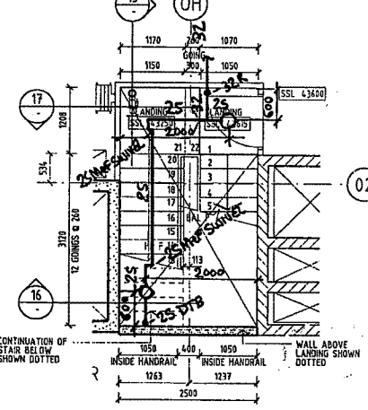
10 LEVEL 02 PLAN STAIR E-02
