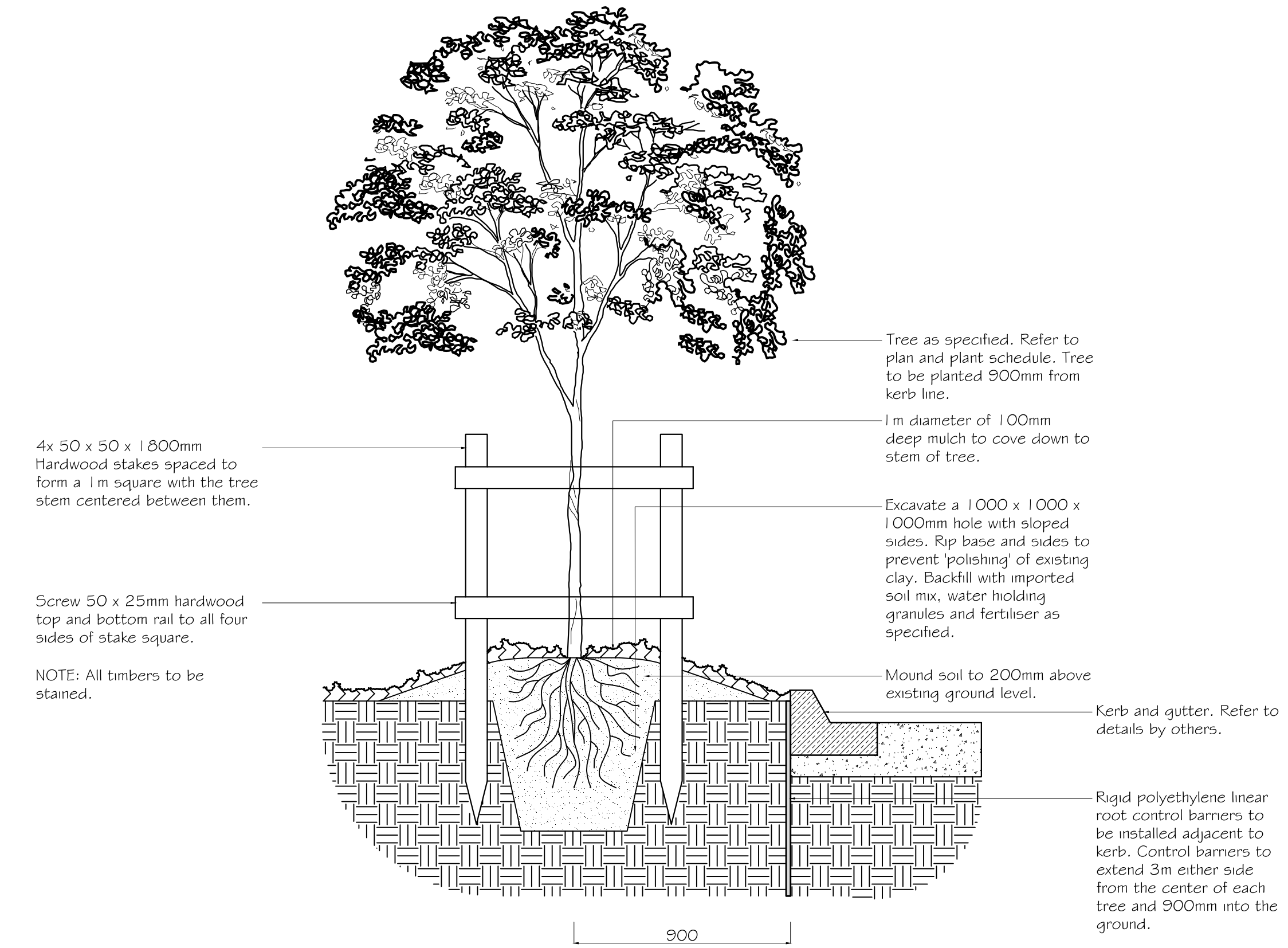
2 STREET TREES IN NATURE STRIP SCALE 1:20 TYPICAL SECTION
