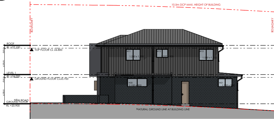
1 WEST ELEVATION 1:250
