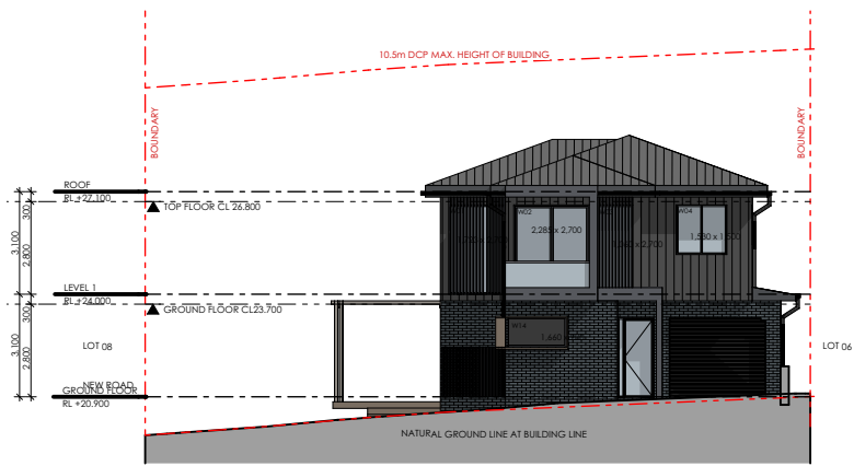
1 WEST ELEVATION 1:250
