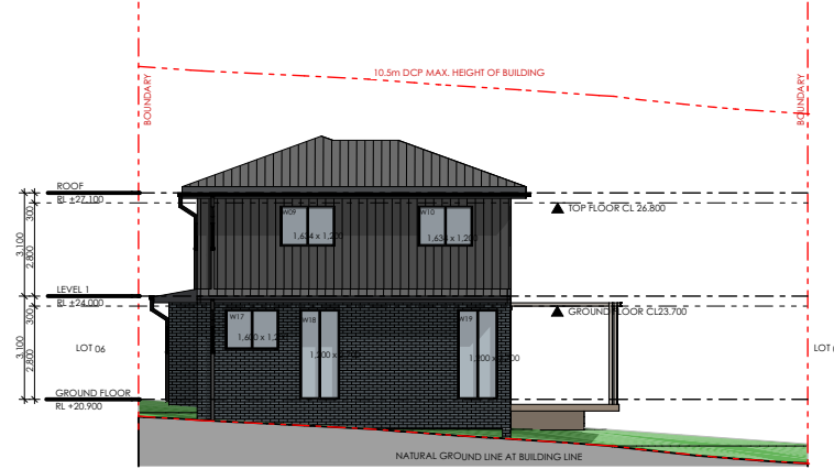
2 EAST ELEVATION 1:250
