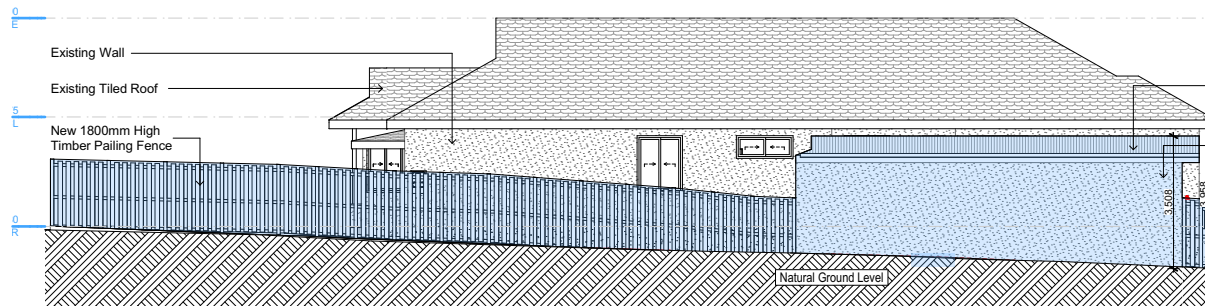
E-02 East 1:200
