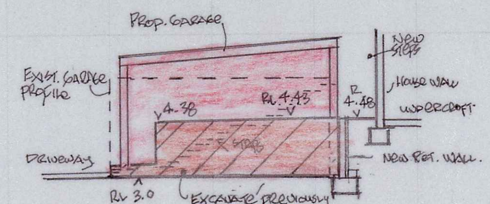
SECTION D - D EXCAVATION
