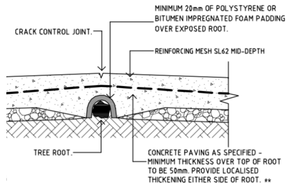
Image B: Example method for bridging concrete surfacing over tree roots provided in the Canterbury Bankstown Council standard drawings. 10
