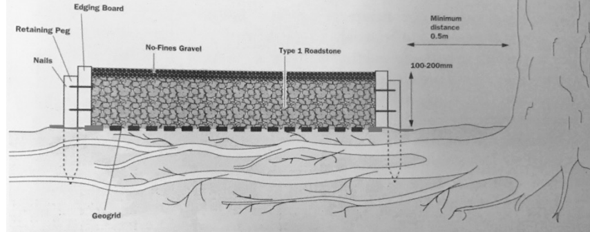
Image A: An image from 'Tree Roots in the Built Environment' 9 , showing how to construct hard surfacing above a trees root system without excavation. Type 1 Roadstones are an example of blue metal or crushed sandstone.
