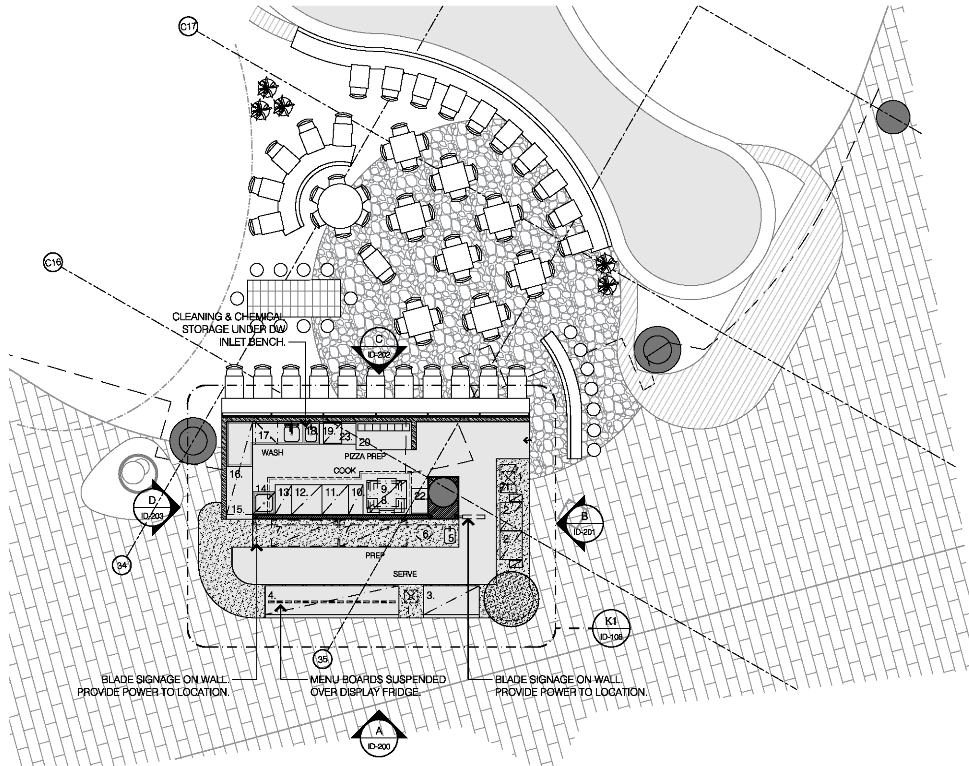
PROPOSED FLOOR PLAN FLOOR PLANS 1:100
