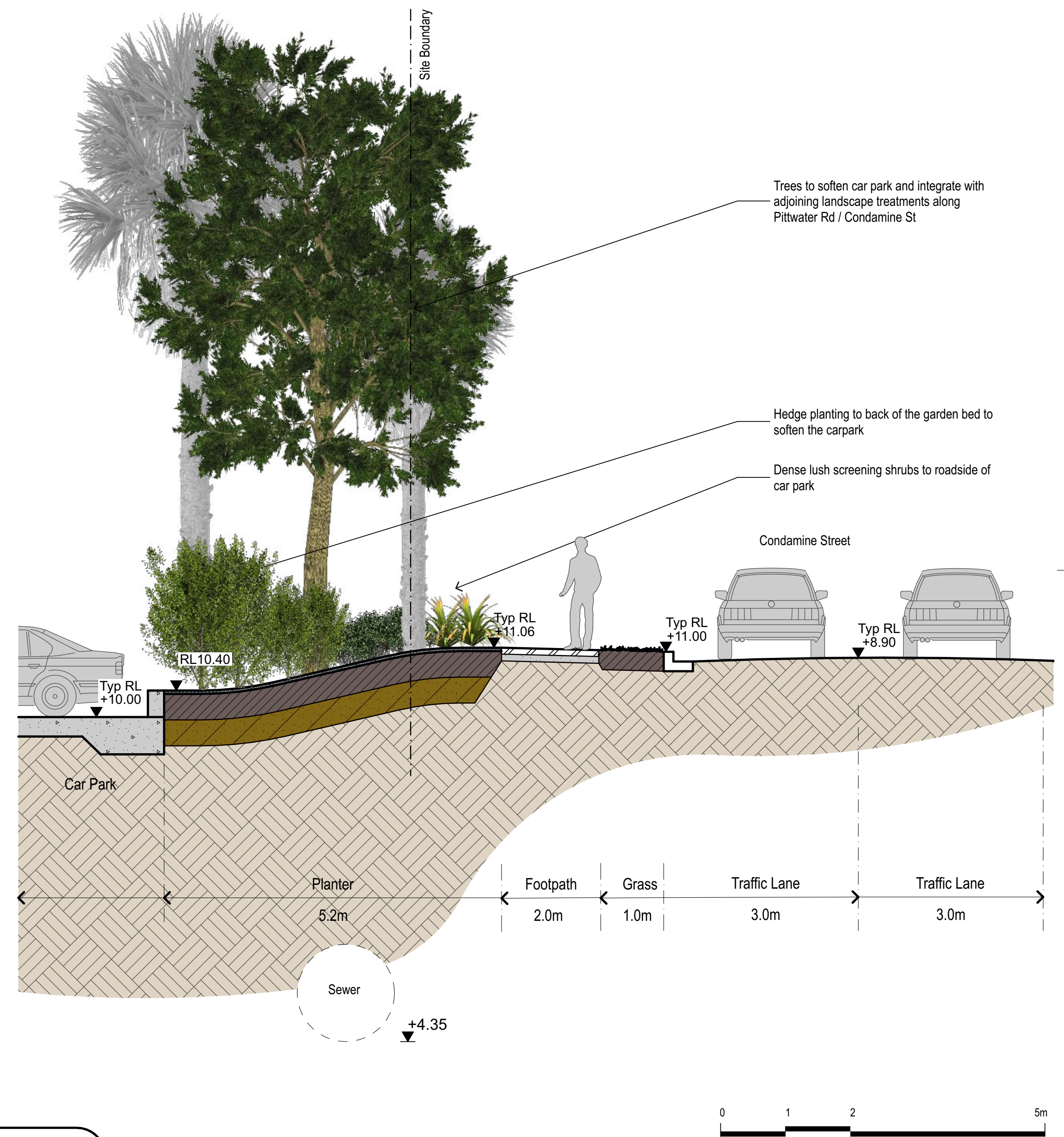
C TYPICAL SECTION - CENTRAL CAR PARKING AREA
