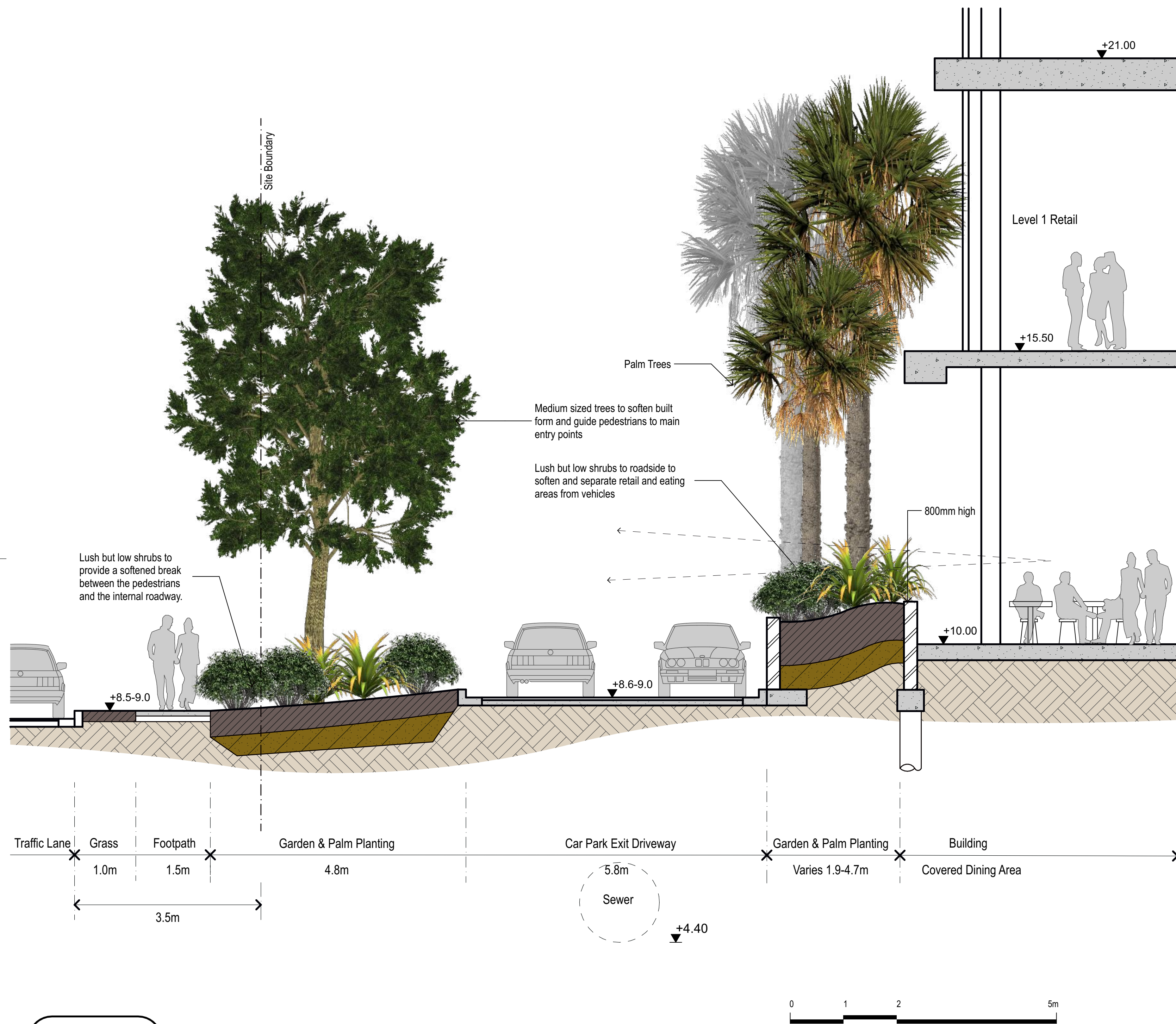
B TYPICAL SECTION - SOUTHERN ENTRY AREA
