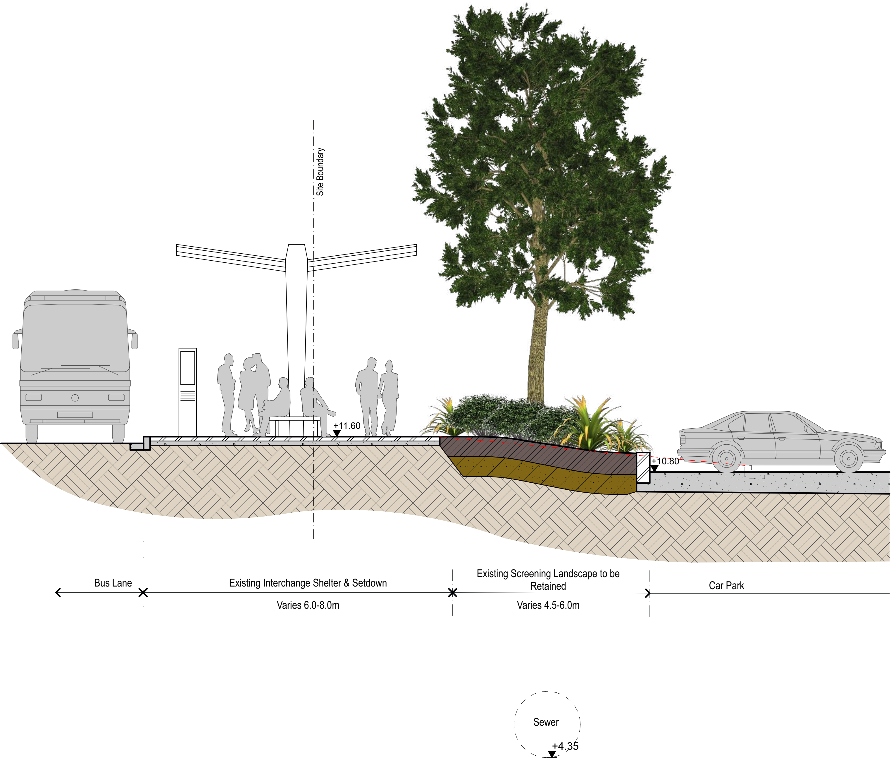
TYPICAL SECTION - NORTHERN BUS INTERCHANGE & CARPARK
